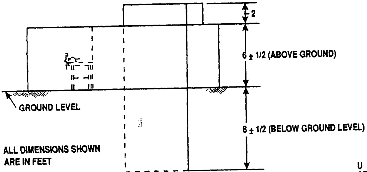
Figure 5-8. Pitch-in barricade.
